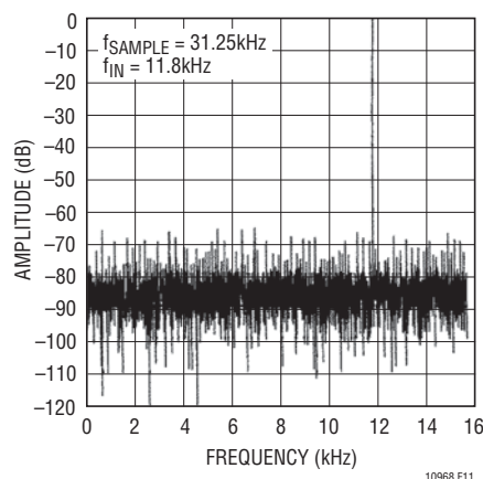
Figure 11. This Clean FFT of an 11.8kHz Input Shows Remarkable Performance for an ADC That Draws Only 100μA When Sampling at the 31.25kHz Rate
