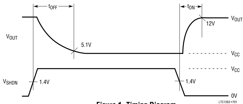
Figure 1. Timing Diagram
