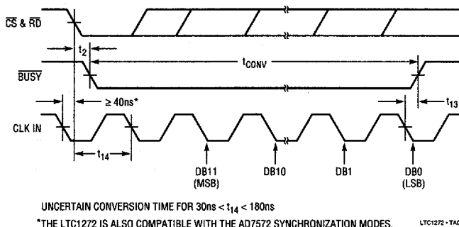
Figure 5. \overline{\text{RD}} and CLK IN for Synchronous Operation
