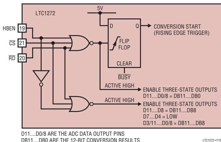
Figure 12. Internal Logic for Control Inputs \overline{\text{CS}} , \overline{\text{RD}} and HBEN
