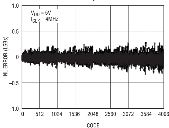
Differential Nonlinearity
