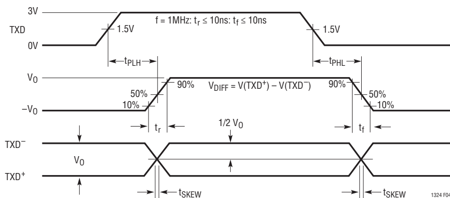
Figure 4. Differential Driver
