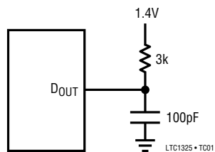
Load Circuit for t_{dD0} , t_r and t_f
