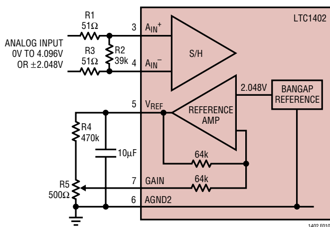
Figure 10a. Full-Scale Adjustment Circuit with \pm 10LSB Range
