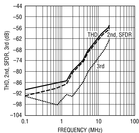
2nd, 3rd and SFDR vs Input Frequency
