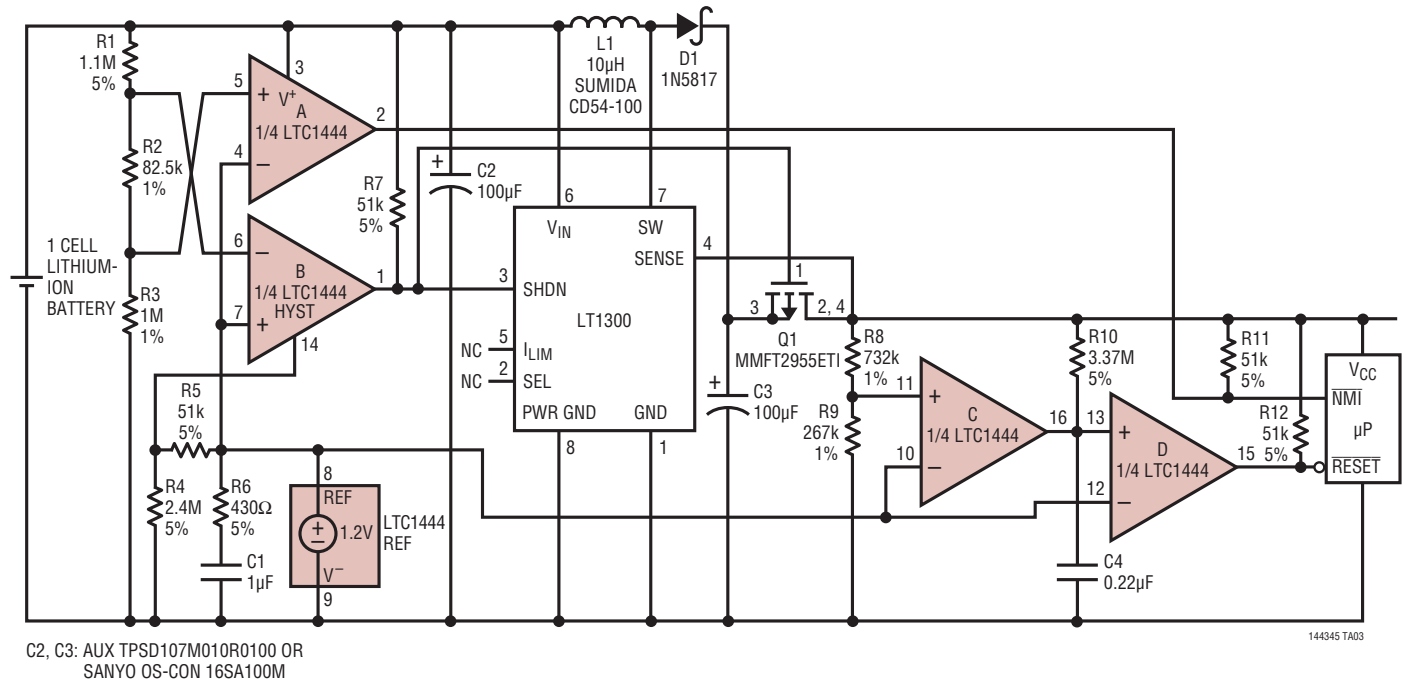
Single Cell to 5V Supply
