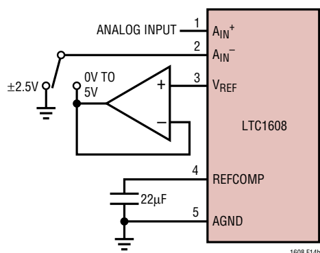
Figure 14b. Selectable 0V to 5V or \pm 2.5\text{V} Input Range
