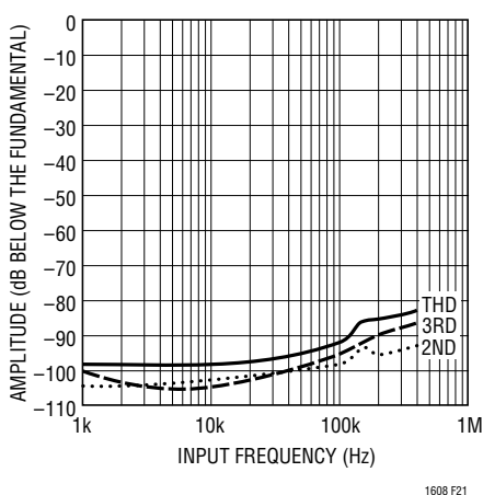
Figure 21. Distortion vs Input Frequency
