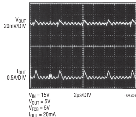
Constant Frequency (Burst Inhibit) Operation (Figure 14)
