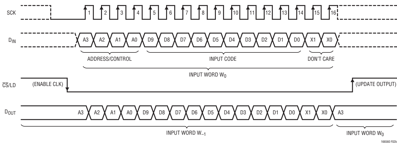
Figure 2b. LTC1660 Register Loading Sequence
