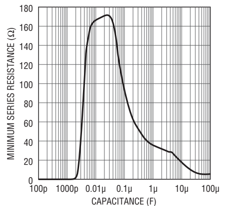
Output Minimum Series Resistance vs Load Capacitance
