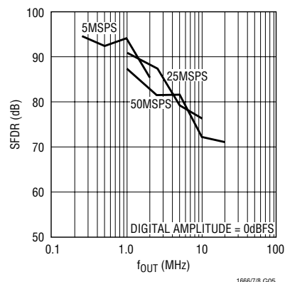
LTC1668 SFDR vs f_{OUT} and f_{CLOCK}
