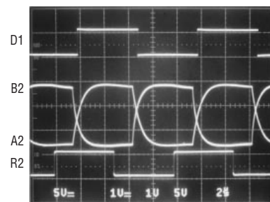
Driving a 1000 Foot STP Cable
