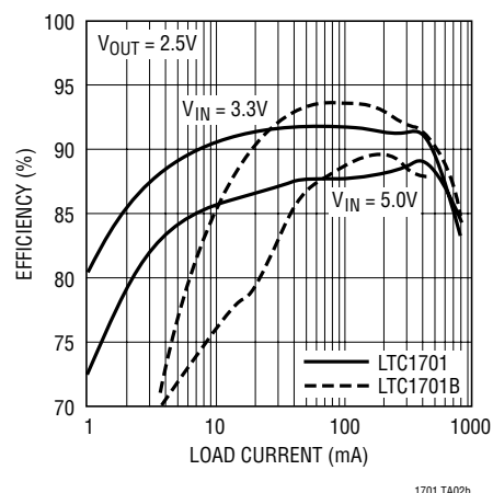
Efficiency Curve
