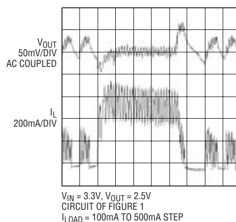
Transient Response
