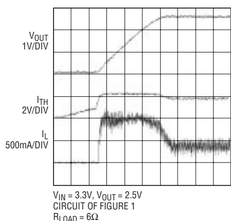
Start-Up
