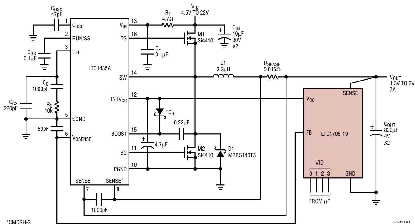
Intel Mobile Pentium II Processor Power Supply
