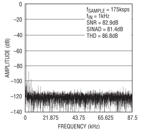
4096 Points FFT Plot ( V_{DD} = 2.7\text{V} , Internal REF)
