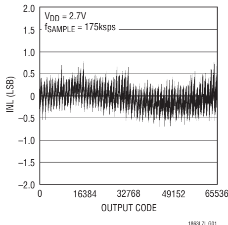
Integral Nonlinearity vs Output Code (LTC1867L)
