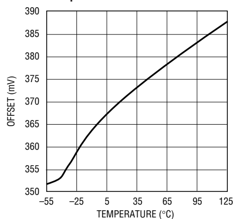
Ramp Offset Voltage vs Temperature
