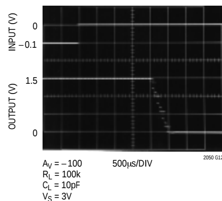
Input Overload Recovery
