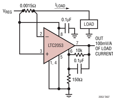
High Side Power Supply Current Sense
