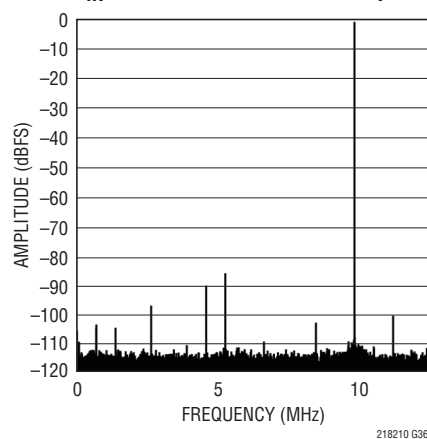
LTC2180: 64k Point FFT, f_{IN} = 140\text{MHz} , -1dBFS, 25MSPS
