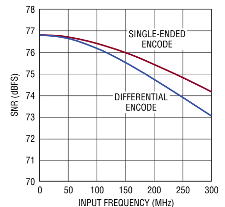
LTC2185: SNR vs Input Frequency, -1\text{dBFS} , 125Msps, 2V Range
