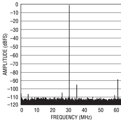
LTC2185: 64k Point FFT, f_{IN} = 30\text{MHz} , -1\text{dBFS} , 125Msps
