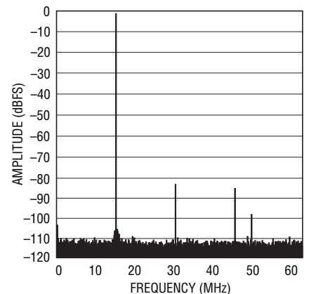
LTC2185: 64k Point FFT, f_{IN} = 140\text{MHz} , -1\text{dBFS} , 125Msps
