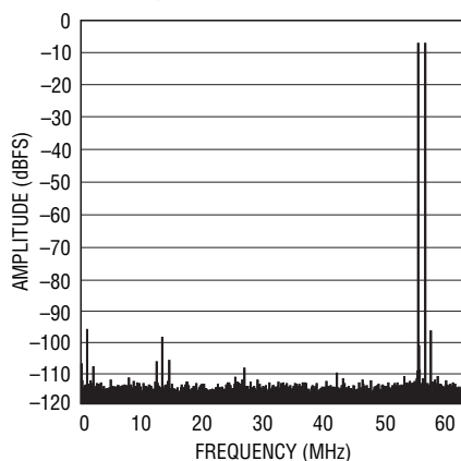
LTC2185: 64k Point 2-Tone FFT, f_{IN} = 69\text{MHz} , 70\text{MHz} , -7\text{dBFS} , 125Msps
