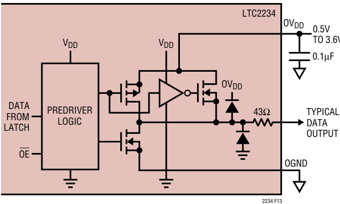
Figure 13. Digital Output Buffer
