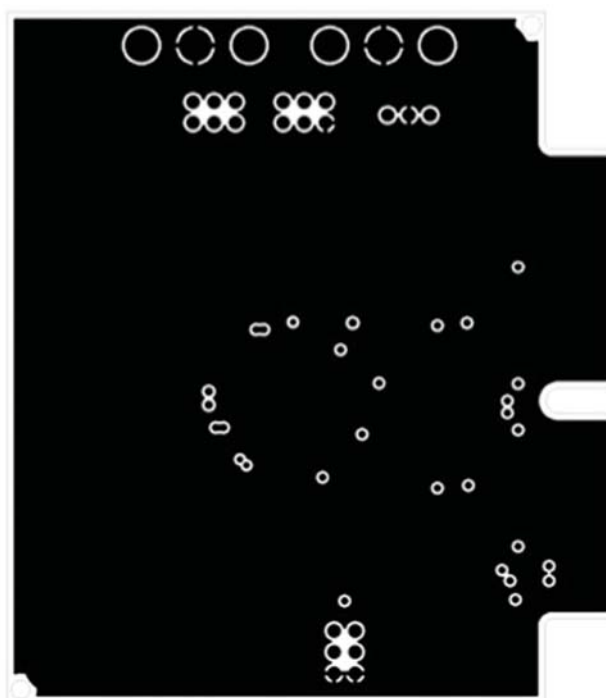
Layer 3 Power/Ground Plane
