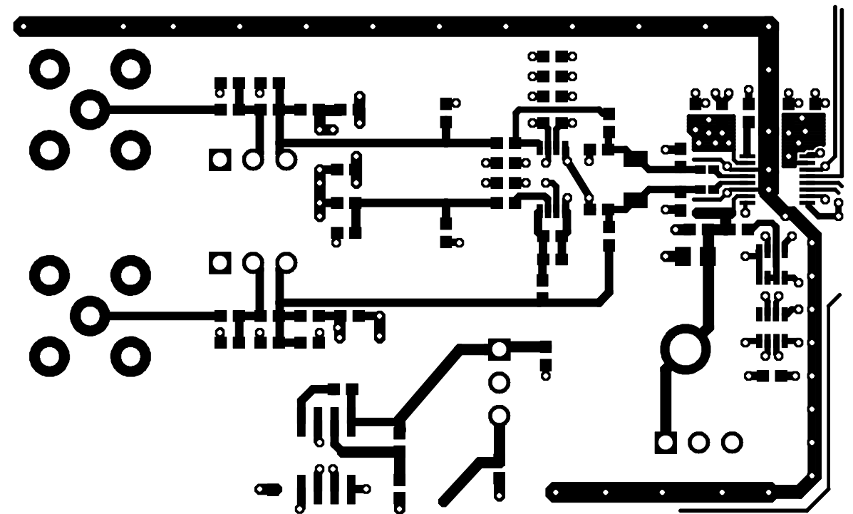
Partial Layer 1 Component Side
