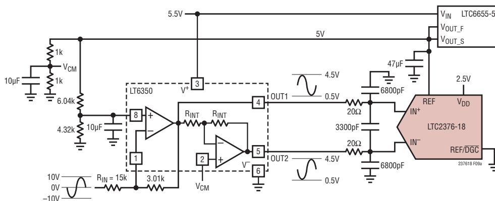
Figure 9a. LT6350 Configured to Accept a \pm 10\text{V} Input Signal While Running Off of a Single 5.5V Supply When Digital Gain Compression Is Enabled in the LTC2376-18
