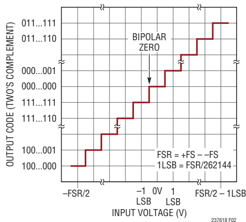
Figure 2. LTC2376-18 Transfer Function
