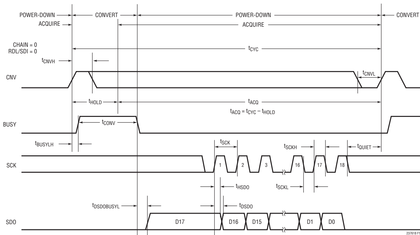
Figure 13. Using a Single LTC2376-18 in Normal Mode
