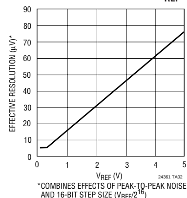
Effective Resolution vs V_{REF}
