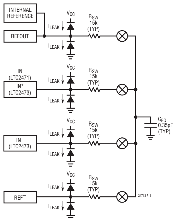
Figure 11. LTC2471/LTC2473 Analog Input/Reference Equivalent Circuit
