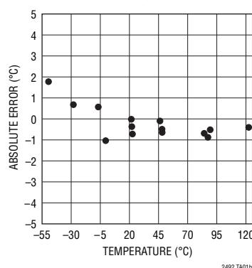
Absolute Temperature Error
