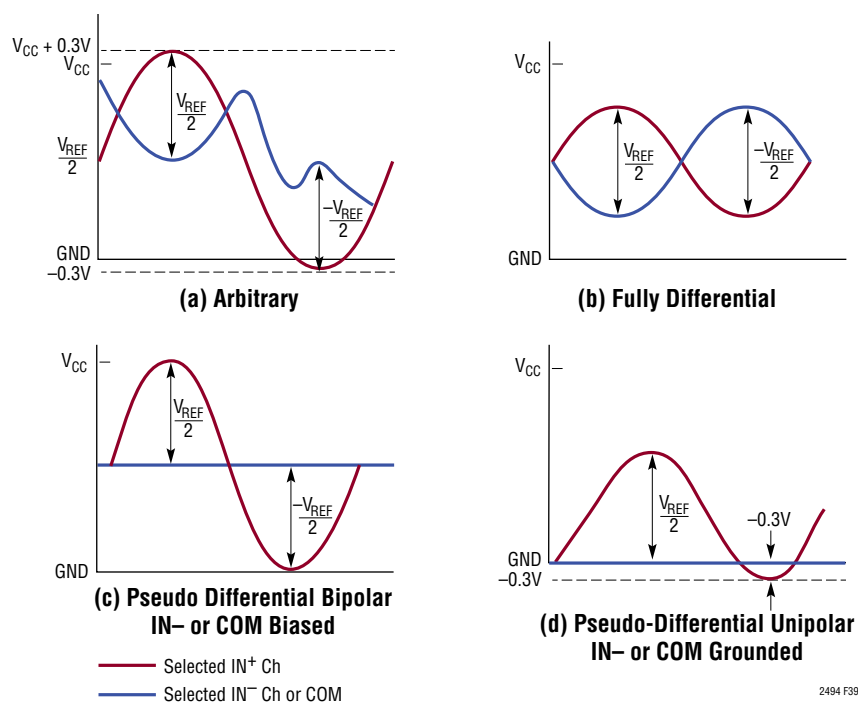
Figure 39. Input Range
