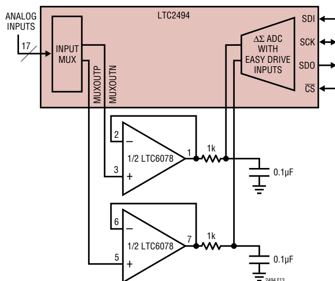
Figure 13. External Buffers Provide High Impedance Inputs and Amplifier Offsets are Automatically Cancelled.
