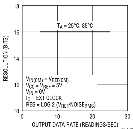
Figure 34. Resolution ( \text{Noise}_{\text{RMS}} \leq 1\text{LSB} ) vs Output Data Rate and Temperature
