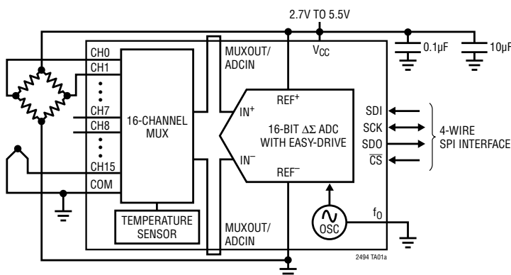
Data Acquisition System with Temperature Compensation
