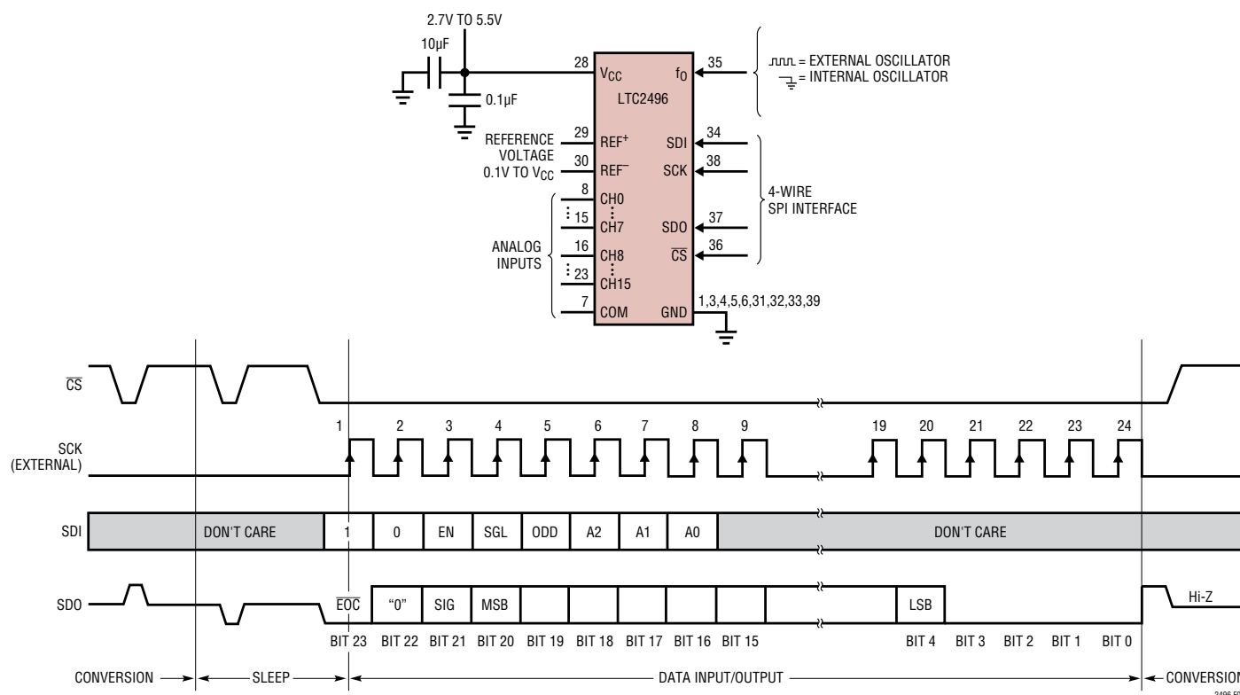
Figure 4. External Serial Clock, Single Cycle Operation
