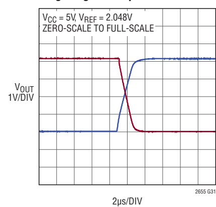
Large-Signal Response
