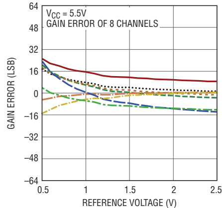
Gain Error vs Reference Input
