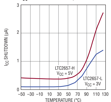
I_{CC} Shutdown vs Temperature
