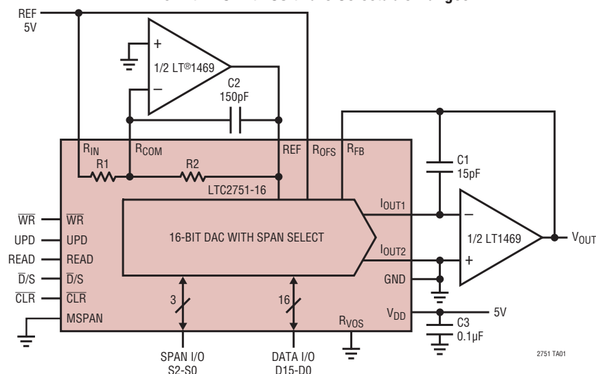
16-Bit DAC with Software Selectable Ranges
