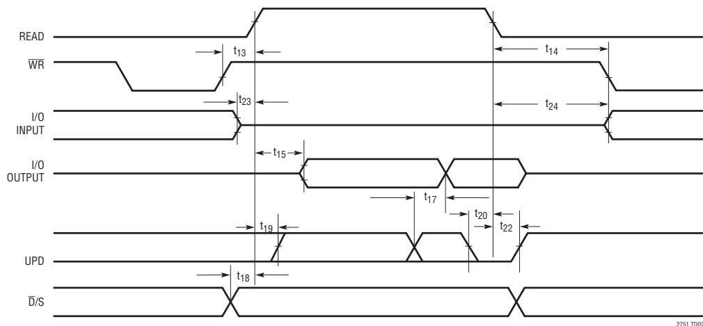
Readback Timing
