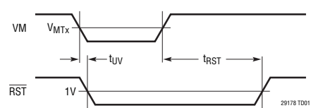
Monitor Input Timing
