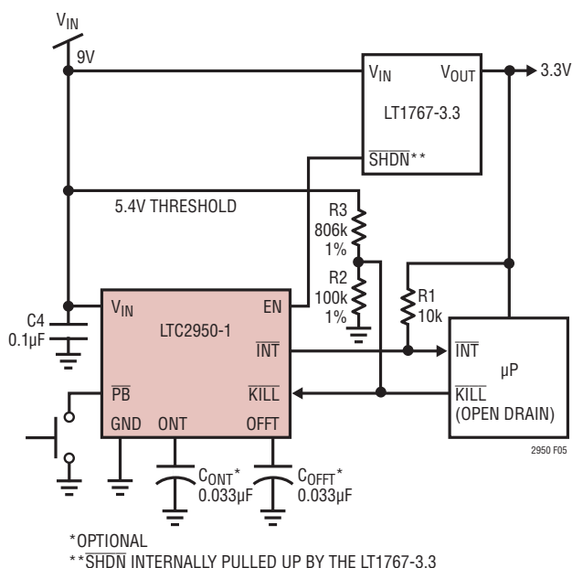
Figure 5. Input Voltage Monitoring with \overline{\text{KILL}} Input
