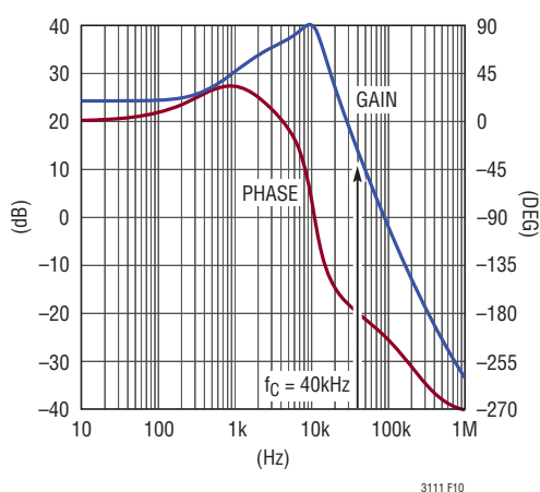
Figure 10. Converter Bode Plot V_{IN} = 3.5\text{V} , V_{OUT} = 5\text{V} , R = 10\Omega
