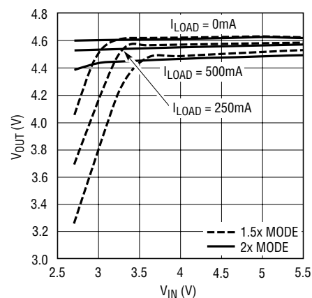
V_{OUT} vs Supply Voltage (4.5V Output Setting)
