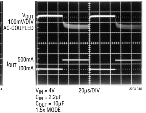
Load Transient (1.5x Mode)
