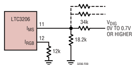
Figure 9. Alternative Digital Brightness Control
