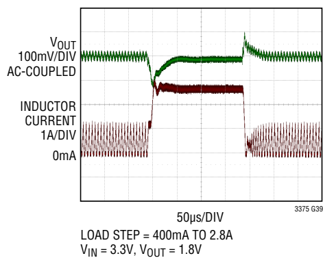
4A Buck Regulator, Transient Response (Burst Mode)
