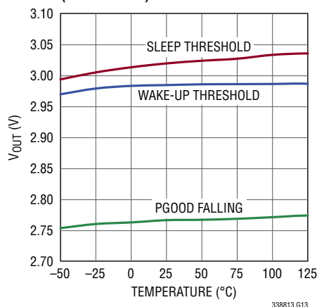
3.0V Output vs Temperature (LTC3388-3)
