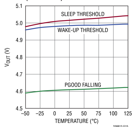
5.0V Output vs Temperature (LTC3388-3)
