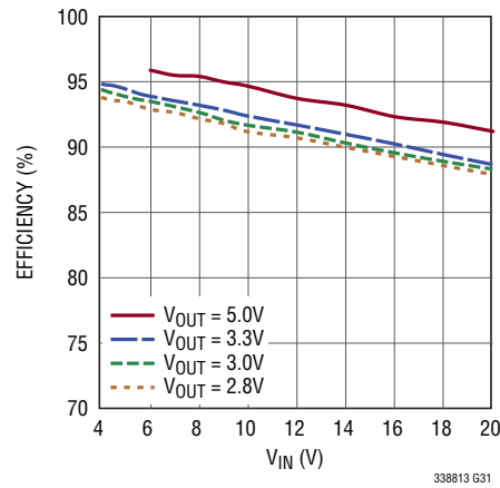
Efficiency vs V_{IN} for I_{LOAD} = 50mA , L = 100\mu H (LTC3388-3)
