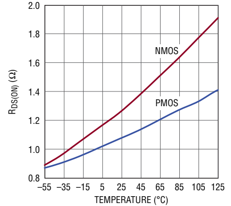
R_{P,BUCK}/R_{N,BUCK} vs Temperature
