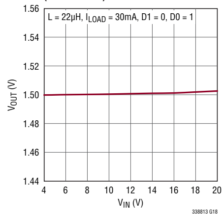
V OUT Line Regulation (LTC3388-1)
