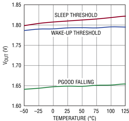
1.8V Output vs Temperature (LTC3388-1)
