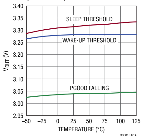
3.3V Output vs Temperature (LTC3388-3)
