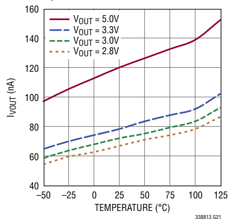
I OUT vs Temperature (LTC3388-3)
