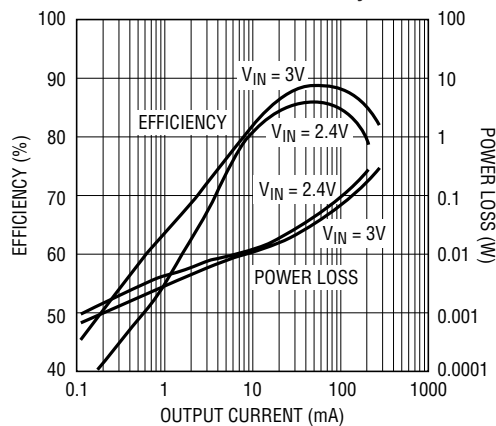
2-Cell to 5V Efficiency
