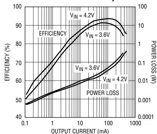
Li-Ion to 5V Efficiency
