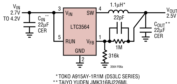
Figure 6a. Typical Application
