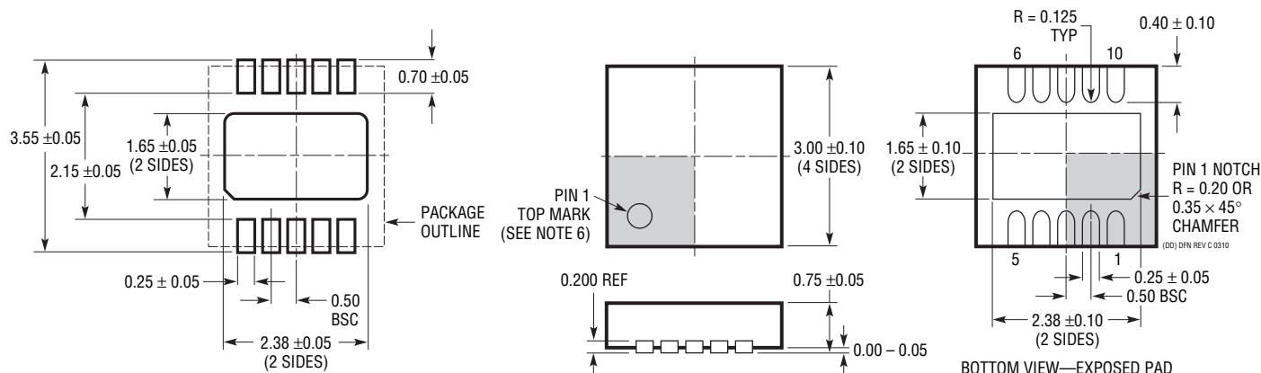
DD Package 10-Lead Plastic DFN (3mm × 3mm) (Reference LTC DWG # 05-08-1699 Rev C)
