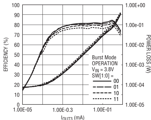
Figure 14. V OUT3 (1.2V) Efficiency and Power Loss vs I OUT3
