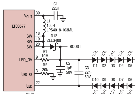
Figure 16. LED Boost Application Circuit
