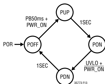
Figure 13. Pushbutton State Diagram
