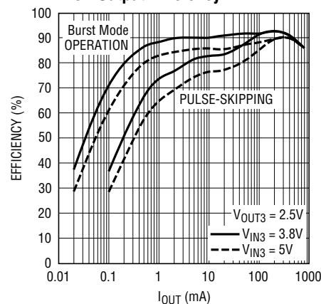
Step-Down Switching Regulator 3 2.5V Output Efficiency
