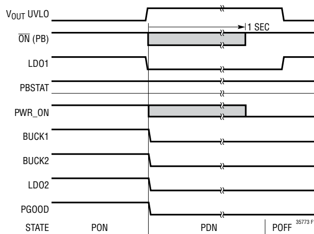
Figure 17. V_{\text{OUT}} UVLO Power-Down
