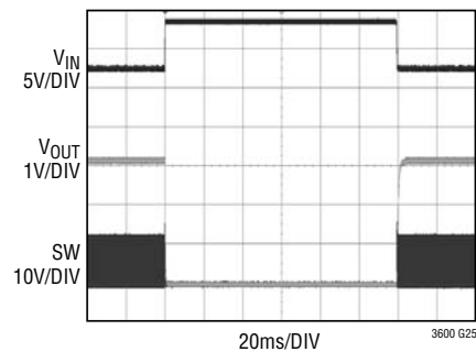
V_{IN} Overvoltage
