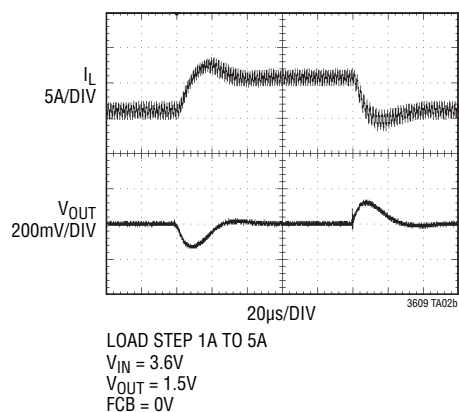
Transient Response
