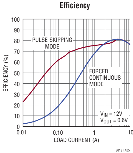
Figure 12. 0.6V, 10A, 200kHz Low Output Voltage Step-Down Converter
