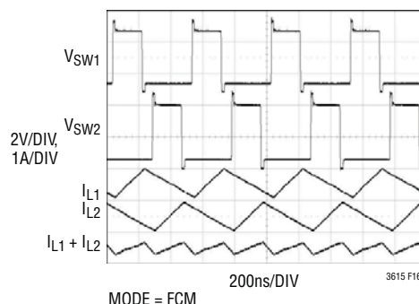
Figure 16. Reduced Ripple Current (Waveform I_{L1} + I_{L2} ) and Ripple Voltage (Not Shown) Through 180° Phase Shift Between SW1 and SW2
